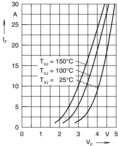
Fig. 1 Max. forward current I_F versus V_F
